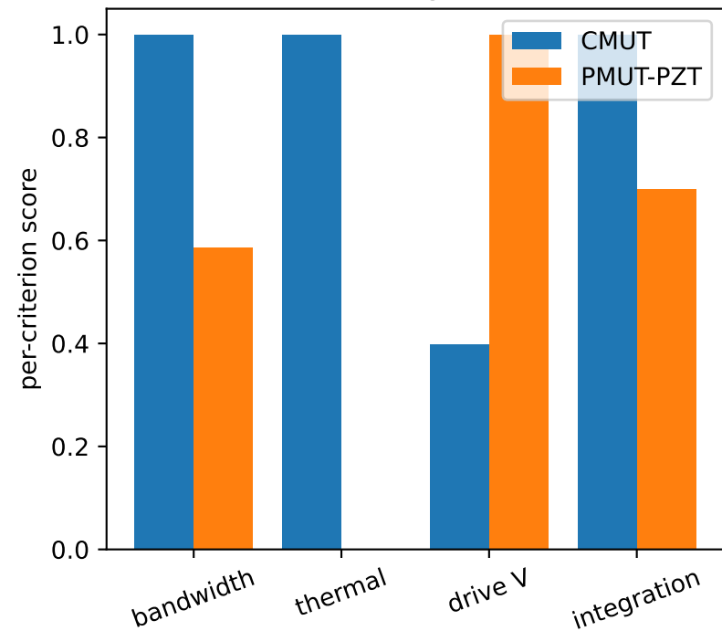
IVUS criteria (higher = better)
