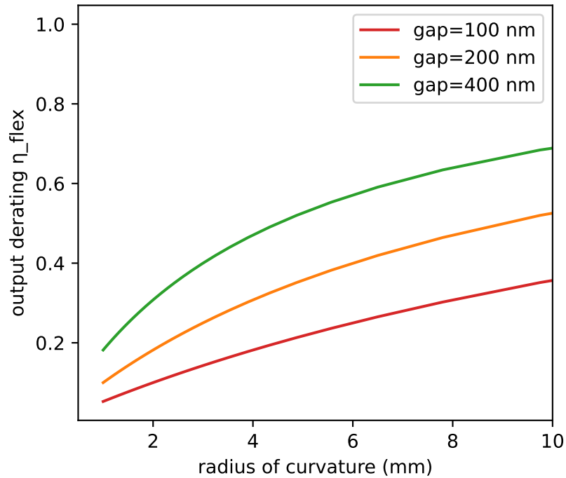
Flexing a CMUT cuts output (tighter gap \rightarrow worse)
