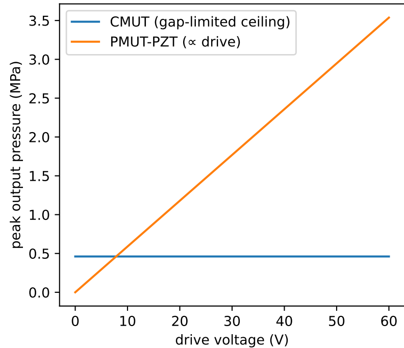
Therapy output: CMUT saturates, PMUT scales
