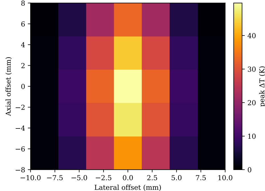
(B) Peak \Delta T /subspot — SEQUENTIAL max 49.7 K
