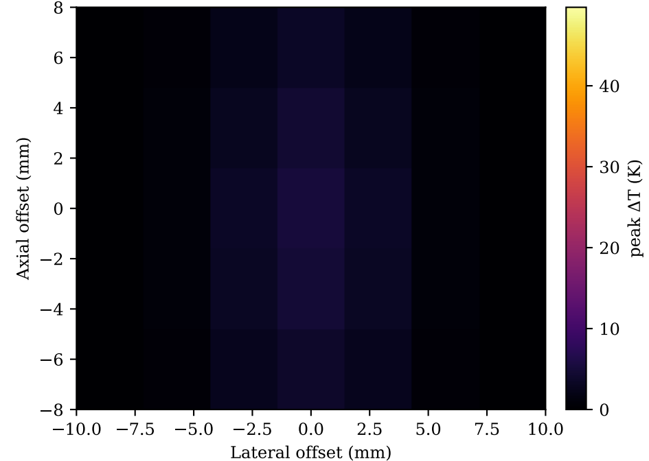
(C) Peak \Delta T /subspot — INTERLEAVED max 5.1 K
