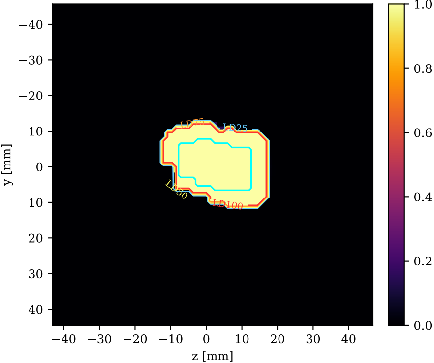
Biologically-effective dose (kill probability + LD iso-contours)
