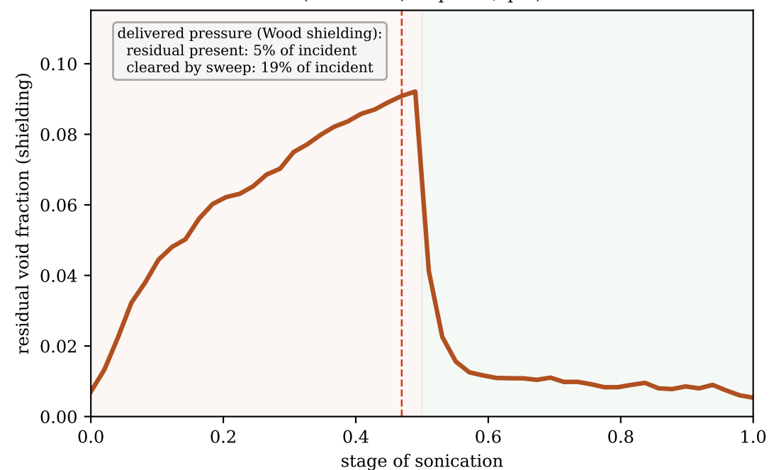
residual built then cleared in wind-down: peak->end 17.2x (PRF 10 Hz, 50 pulses/spot)
