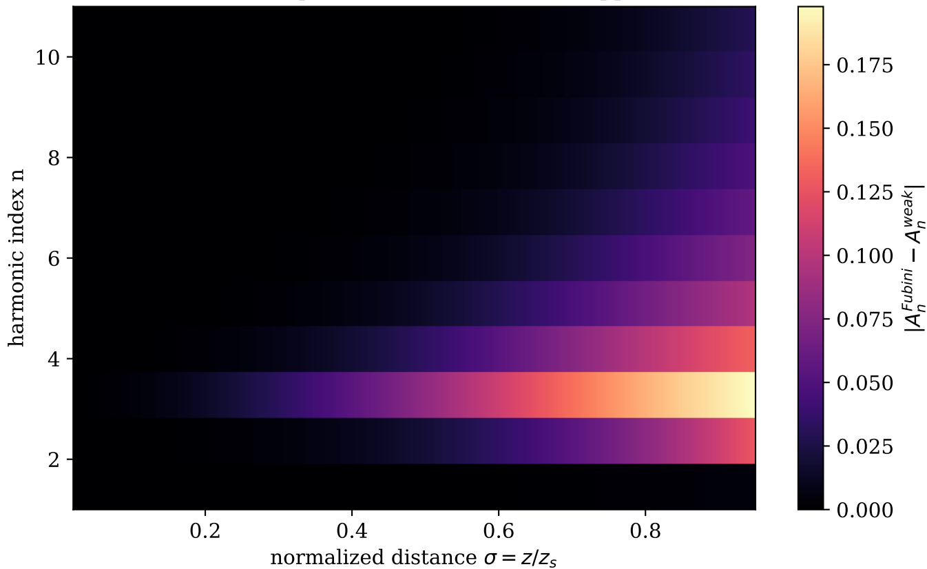
Fubini harmonic departure from weak-shock approximation
