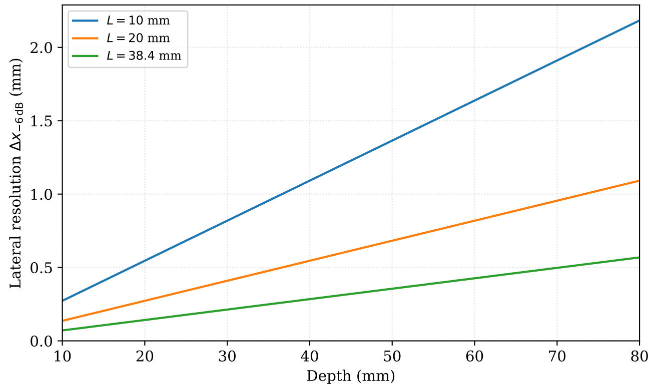
Lateral Resolution vs Depth (Eq. 4.12, f_0 = 5 MHz, uniform apodization)
