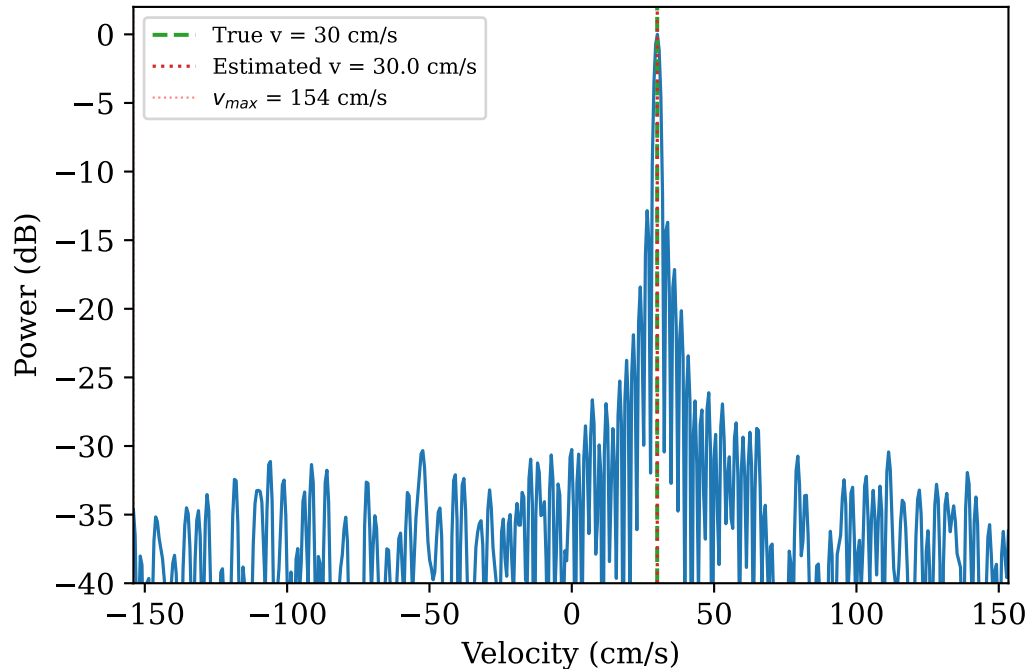
Doppler Spectrum — f_0 = 5 MHz, \alpha = 60.0^\circ
