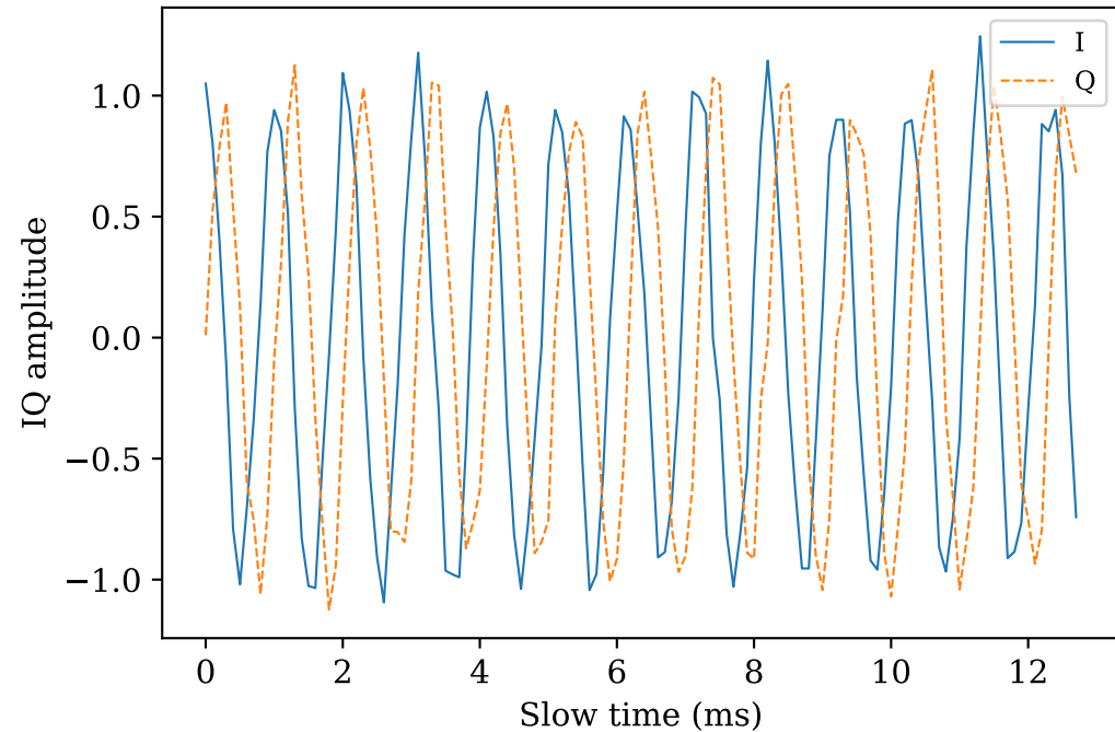
Slow-time IQ signal (single scatterer)
