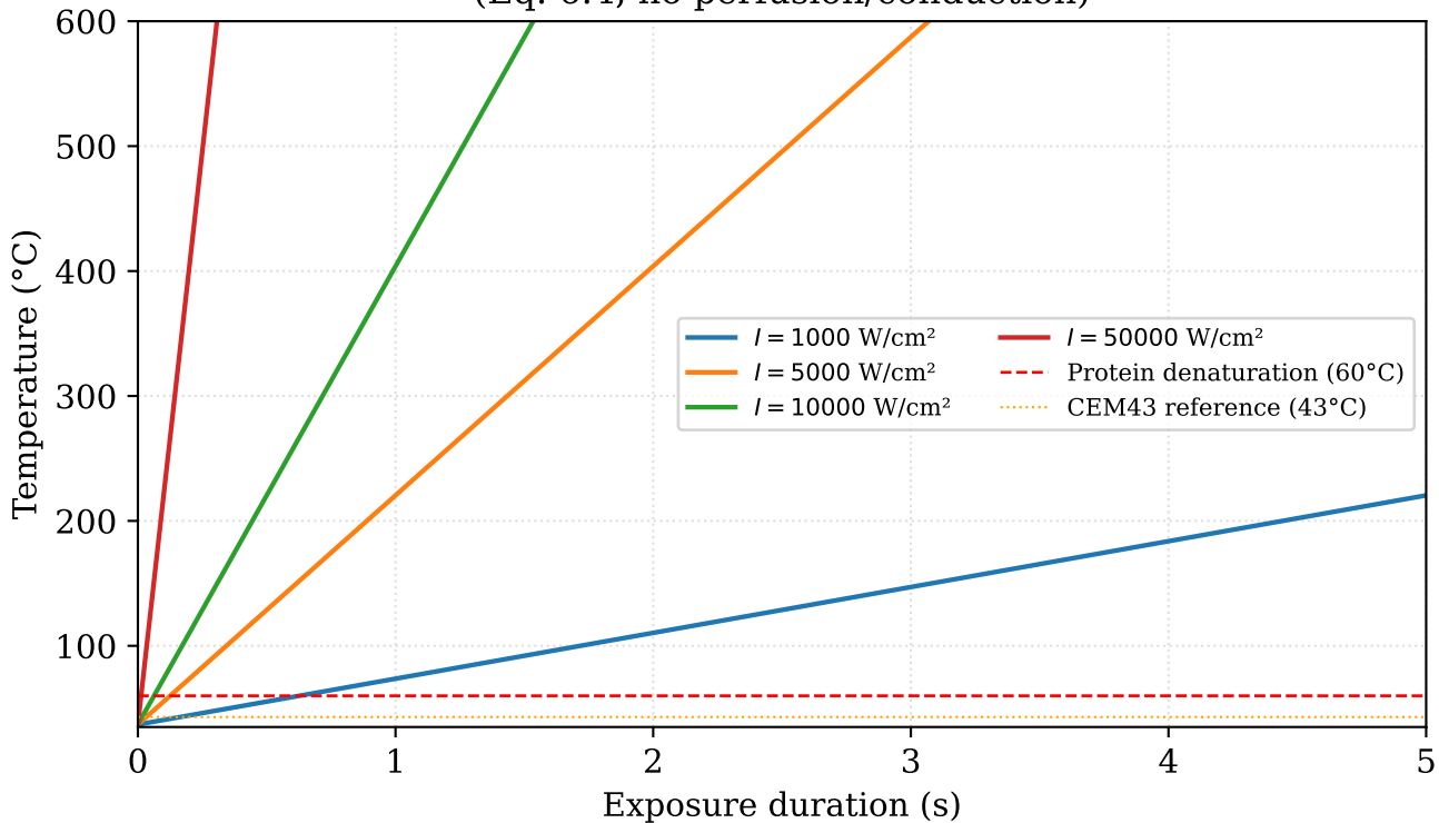
Focal Temperature Rise — Liver Tissue, f_0 = 1 MHz (Eq. 6.4, no perfusion/conduction)
