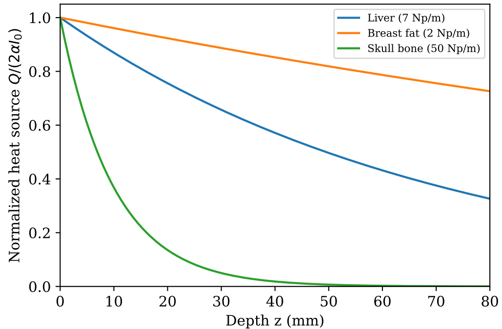
Volumetric Power Deposition (Eq. 6.1)
