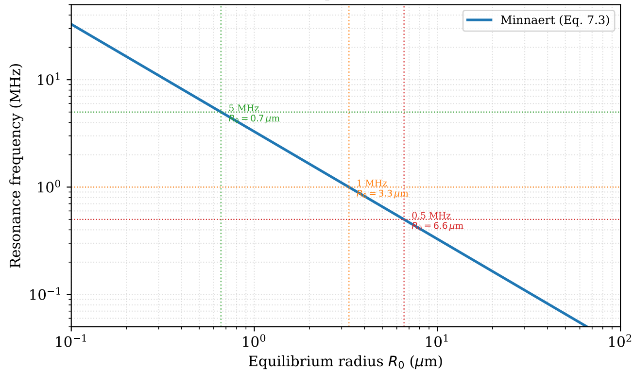
Minnaert Resonance (Eq. 7.3) — Gas Bubble in Water
