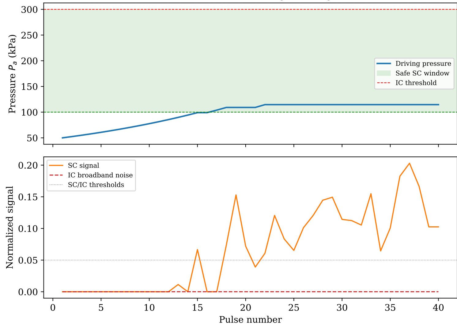
PCD-Feedback Controller Convergence (Algorithm 7.1)
