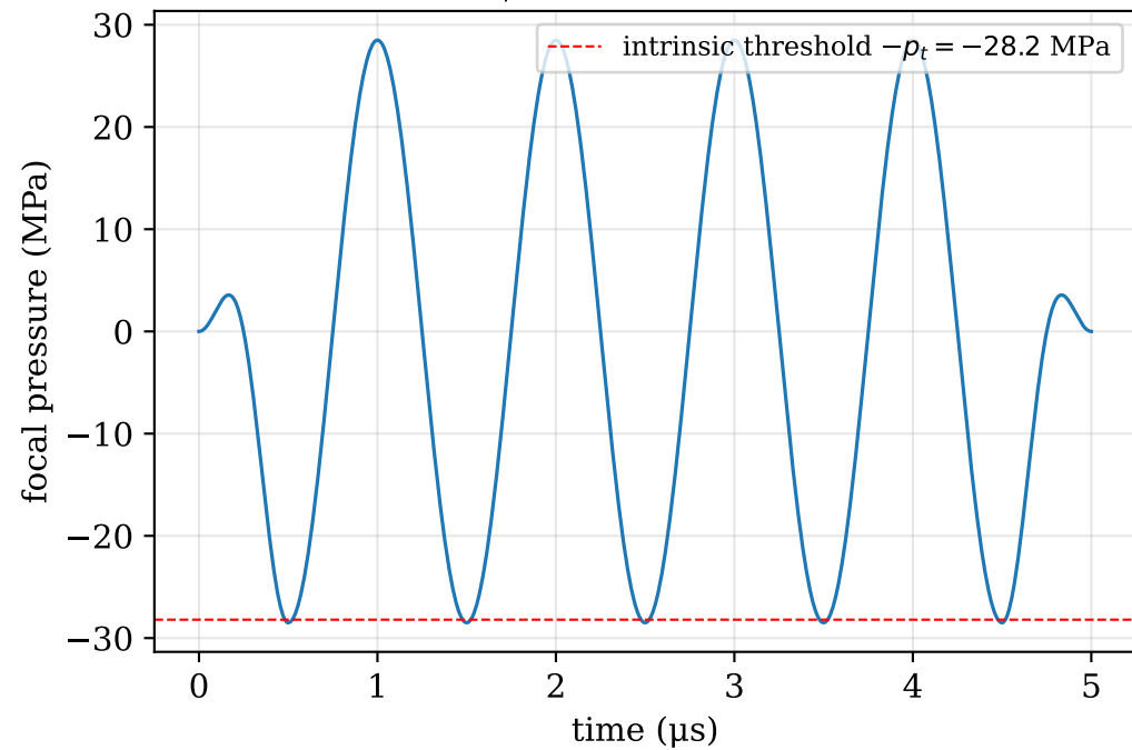
Classical: \tau_p = 5 \mu\text{s} , PNP = -28.5 \text{ MPa}
