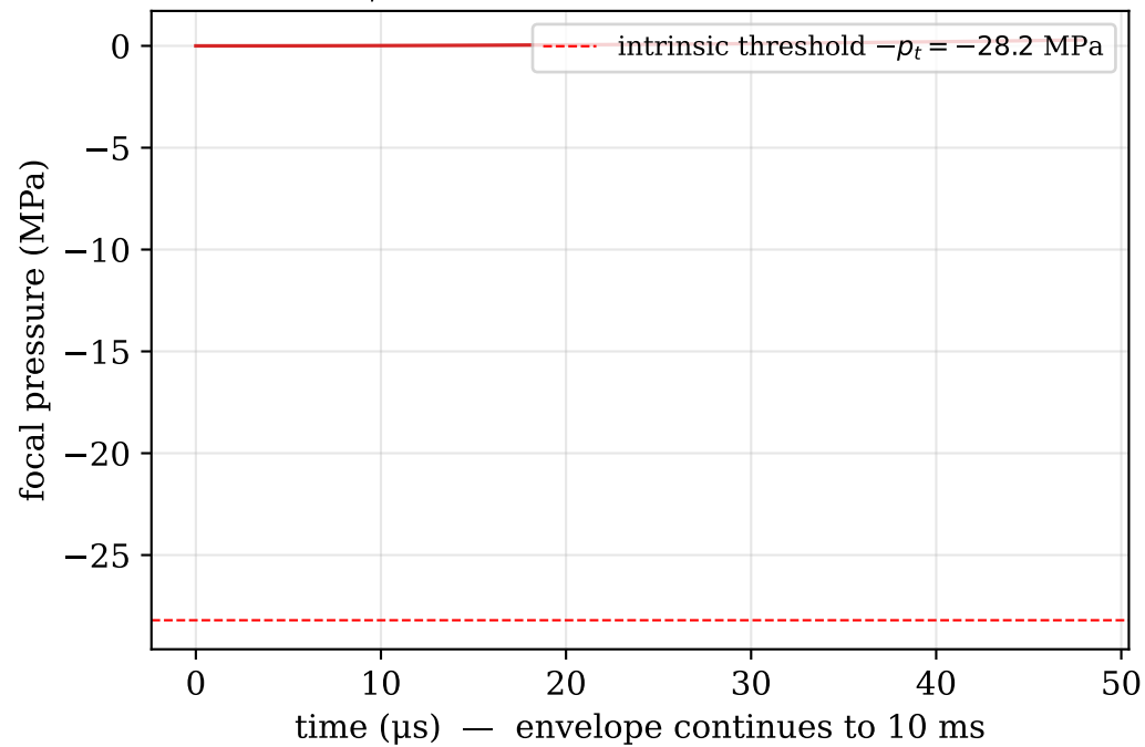
Millisecond: \tau_p = 10 \text{ ms} , PNP = -17.0 \text{ MPa} , PPP = 80 \text{ MPa}
