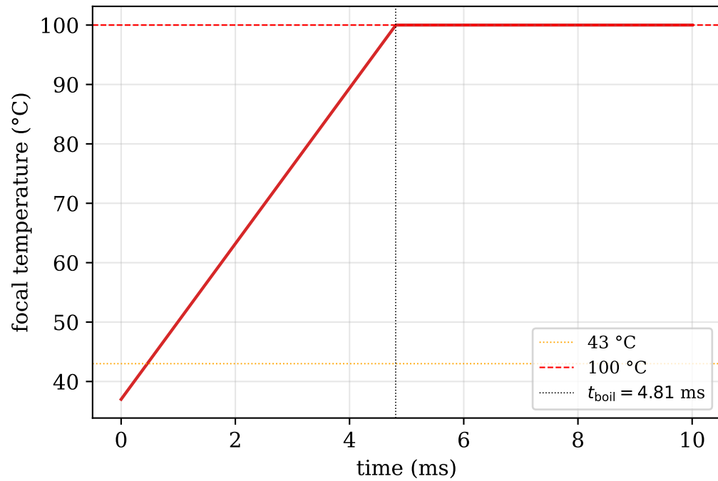
Millisecond, peak T = 100 \text{ }^{\circ}\text{C}
