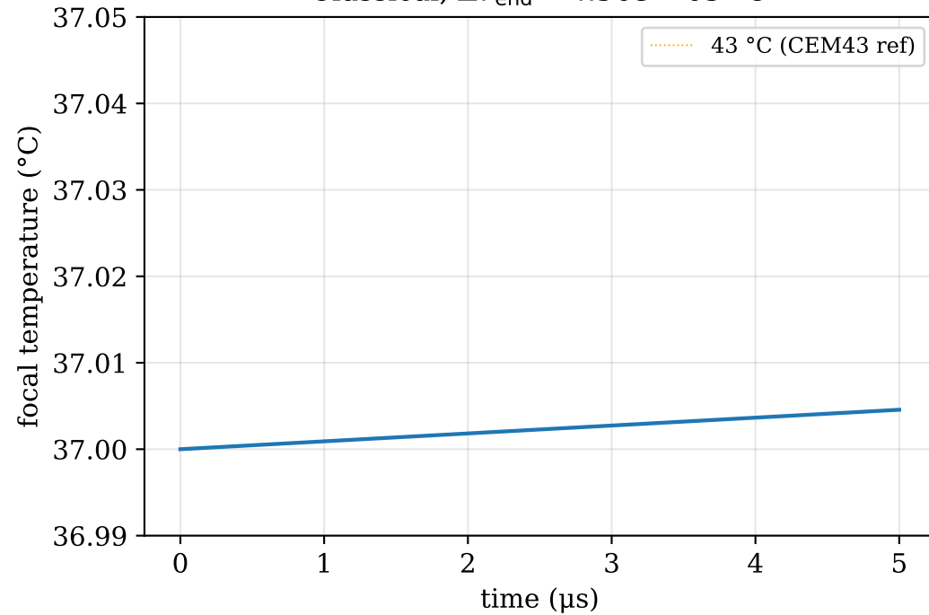
Classical, \Delta T_{\text{end}} = 4.56e - 03 \text{ }^{\circ}\text{C}
