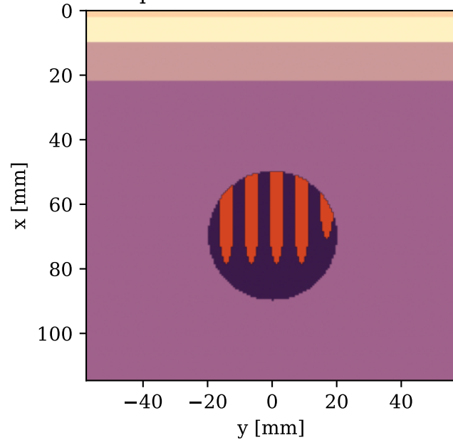
ms sub-threshold cavitation (500 kHz, 18 MPa, 5 ms) predicted ablation lesion
