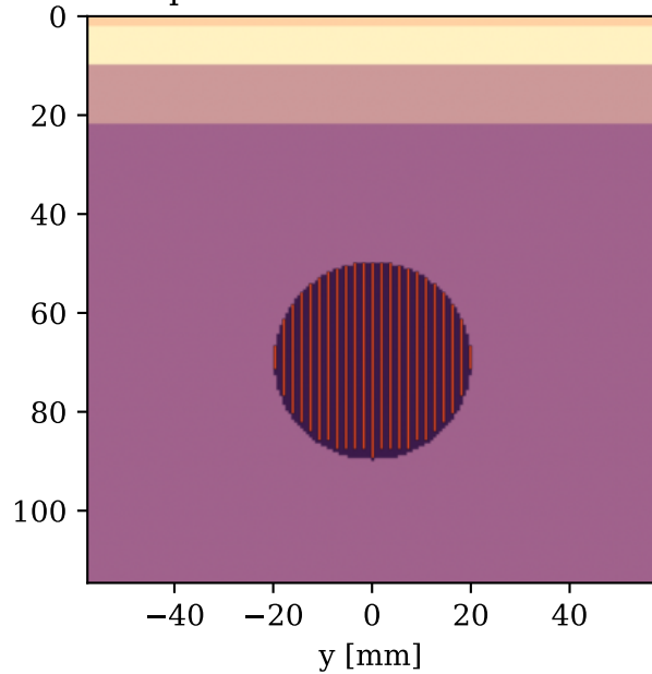
us intrinsic-threshold (1 MHz, 30 MPa) predicted ablation lesion
