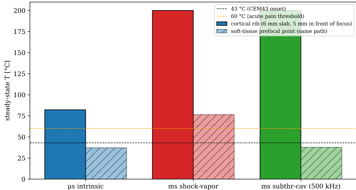
Bone-adjacent thermal safety: rib heating per scenario
