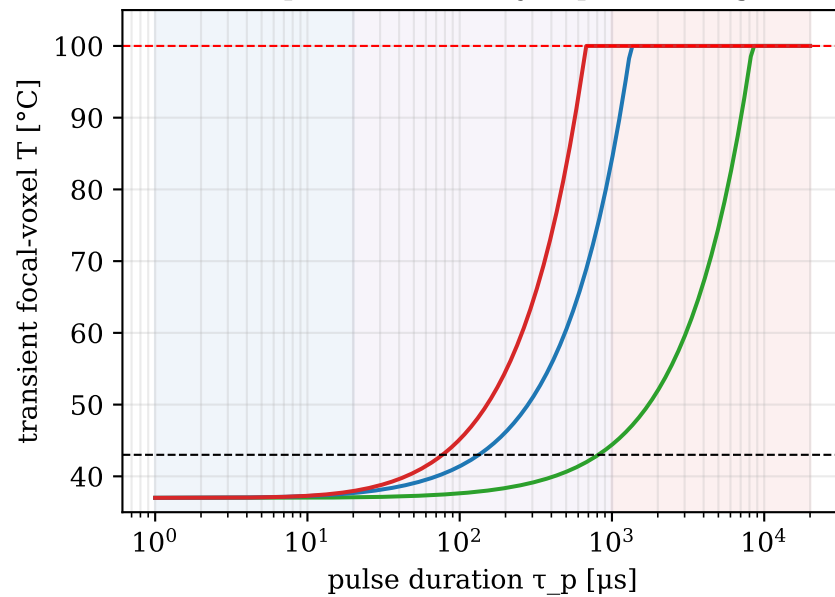
Transient focal-voxel temperature (clamped at 100 °C by vapor seeding)
