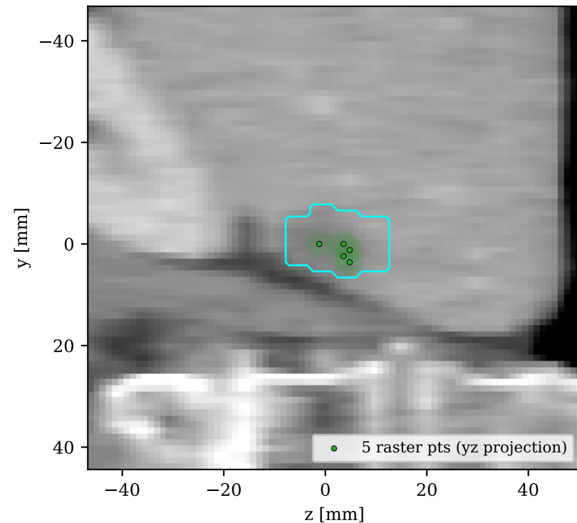
ms sub-threshold cav (500 kHz, 18 MPa, 5 ms) raster: 5 pts \times 5.2 mm FWHM-lat, 0.1 min
