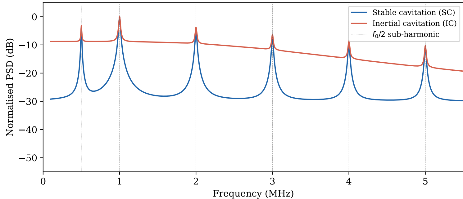
Cavitation emission spectra SC: harmonic lines; IC: elevated broadband floor
