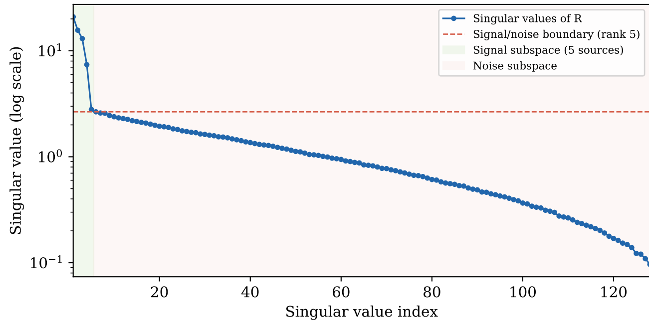
Cross-spectral density matrix singular values Eigenspace PAM uses signal subspace to improve spatial resolution
