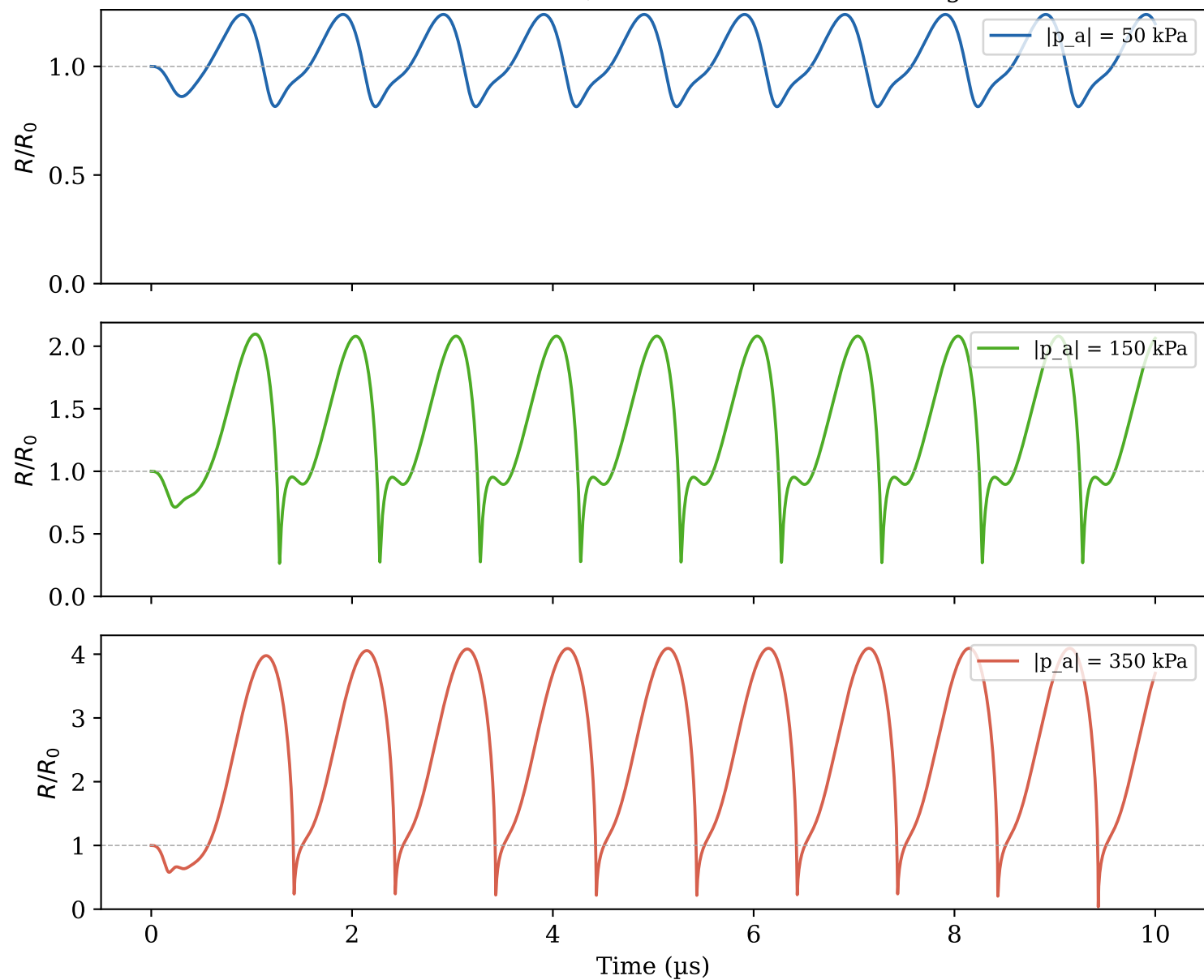
Keller-Miksis MB dynamics — R_0 = 1.5 \text{ }\mu\text{m} , f_0 = 1 \text{ MHz} SonoVue-like shell; LIFU sub-threshold driving
