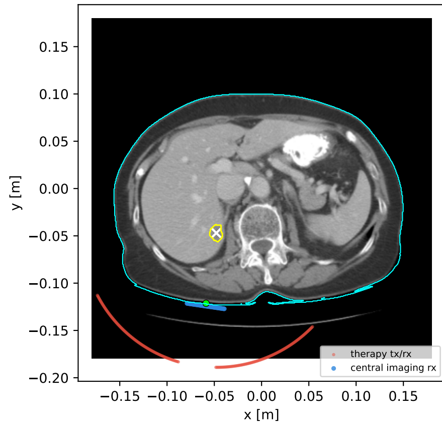
liver: HistoSonics-like skin arc full CT slice, 256 elements, skin gap 3.0 mm
