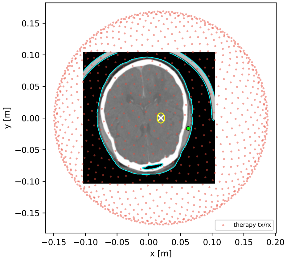
brain: INSIGHTEC-like helmet full CT slice, 1024 elements, helmet clearance 15.0 mm
