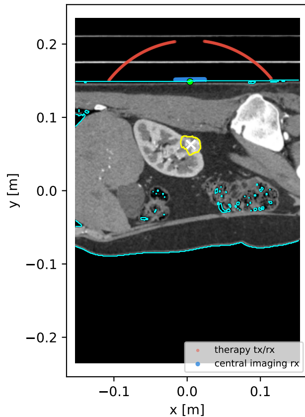
kidney: HistoSonics-like skin arc full CT slice, 256 elements, skin gap 3.0 mm
