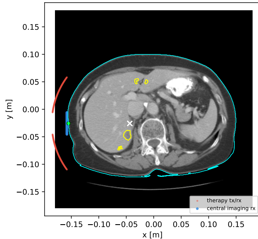
liver: HistoSonics-like skin arc full CT slice, 256 elements, skin gap 3.0 mm
