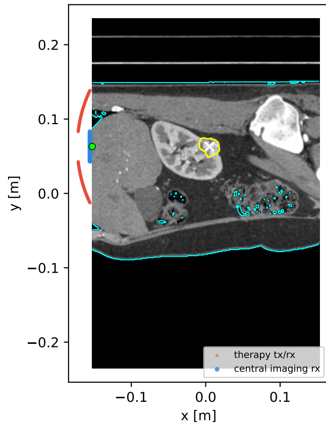
kidney: HistoSonics-like skin arc full CT slice, 256 elements, skin gap 3.0 mm
