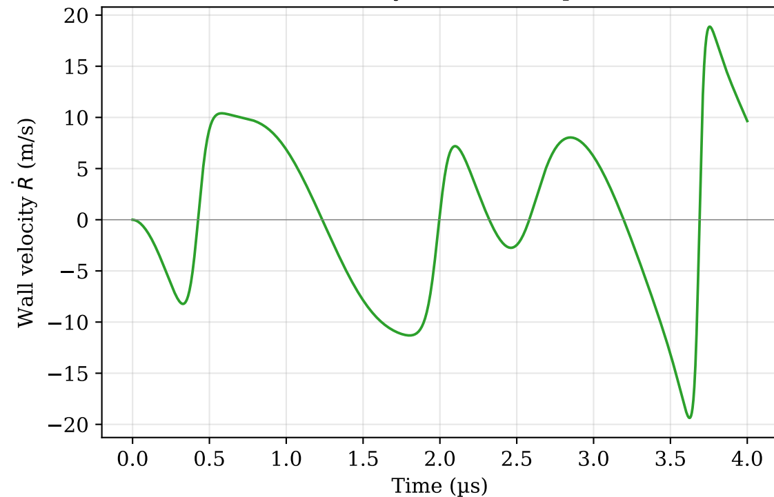
Gilmore wall velocity (inertial collapse/rebound)
