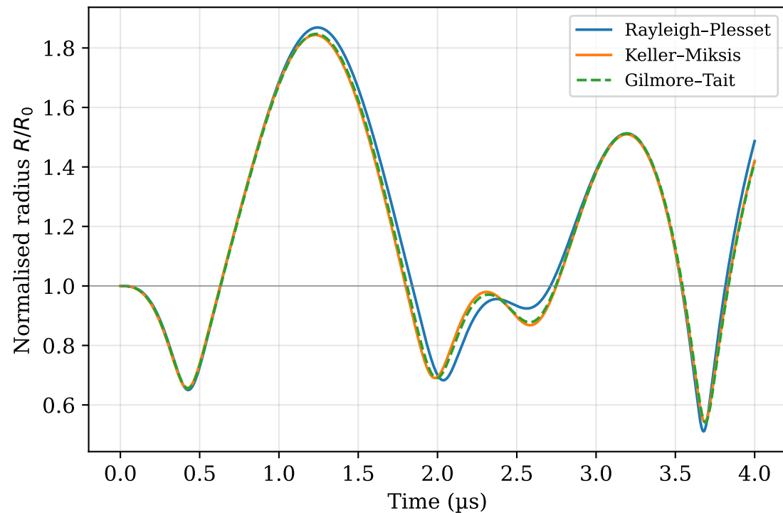
Bubble response — R_0 = 5\text{ }\mu\text{m} , 1 MHz, 200 kPa
