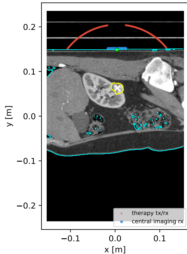
kidney: skin-coupled histotripsy arc full CT slice, 256 elements, skin gap 3.0 mm
