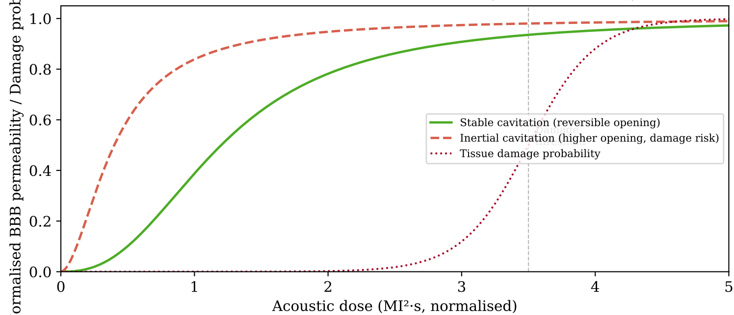
BBB permeability vs acoustic dose Hill model fit to Evans-blue extravasation (McDannold 2008)
