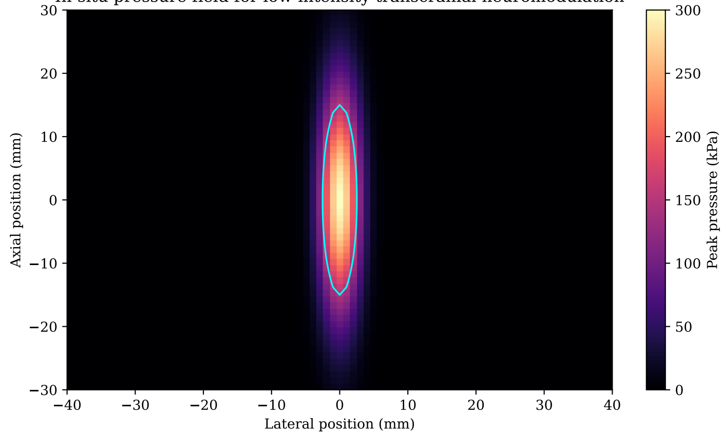
In-situ pressure field for low-intensity transcranial neuromodulation
