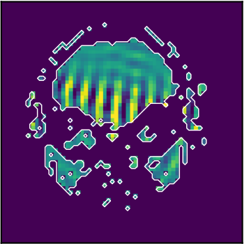
subharmonic
