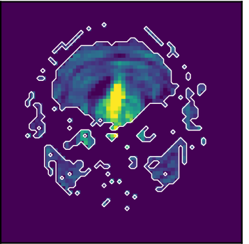
normal FWI
