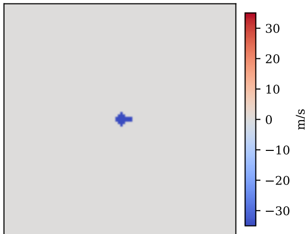
lesion delta c
