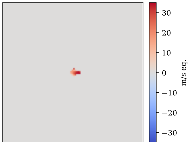
nonlinear susceptibility
