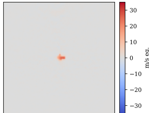
nonlinear FWI
