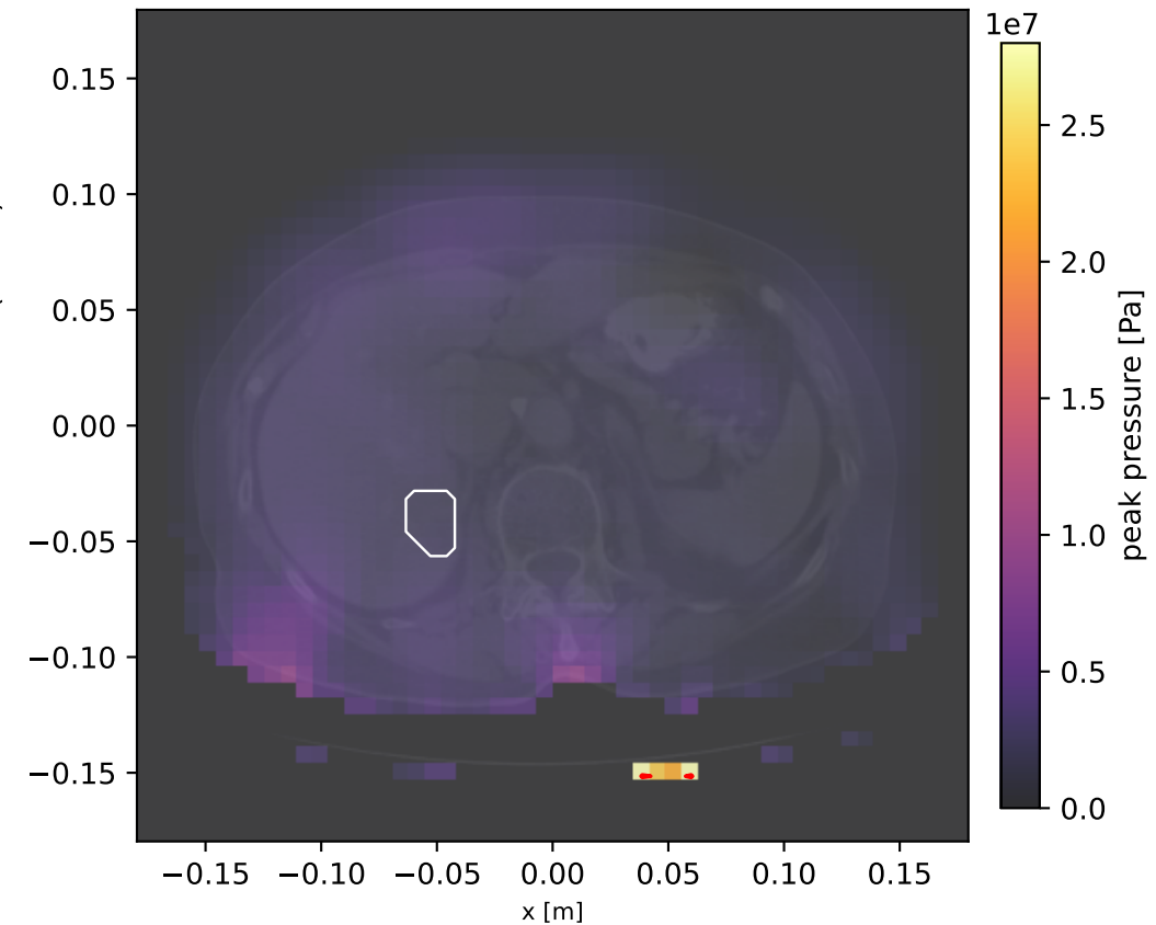
Focused-US peak-pressure exposure red: intrinsic-threshold cavitation isoline (26 MPa)
