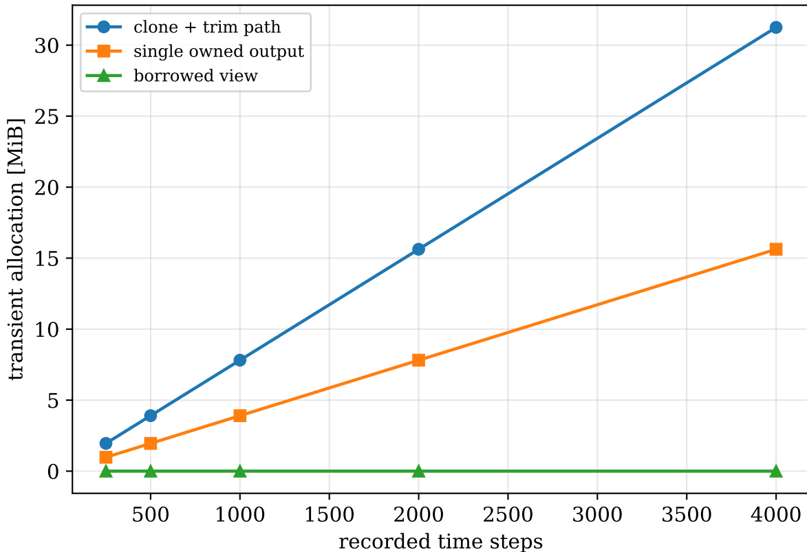
Sparse recorder extraction memory invariant
