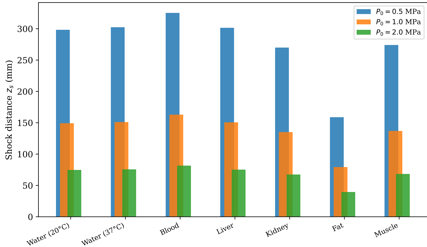
Shock Distance vs Medium — f_0 = 1 MHz (Eq. 3.28)
