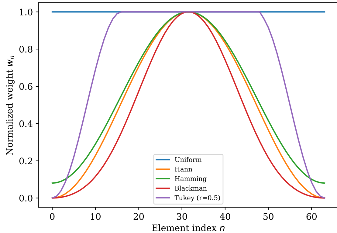
Apodization Windows
