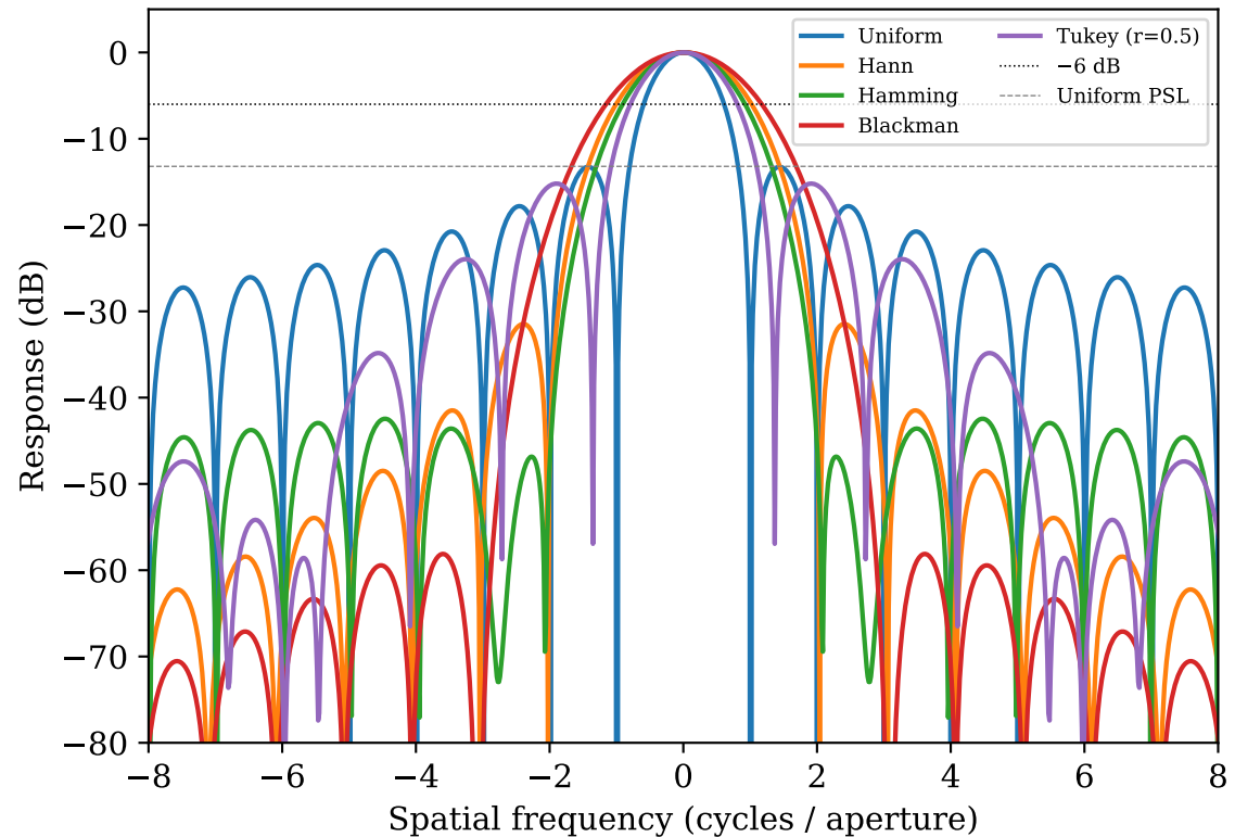
Frequency Response (sidelobe envelope)
