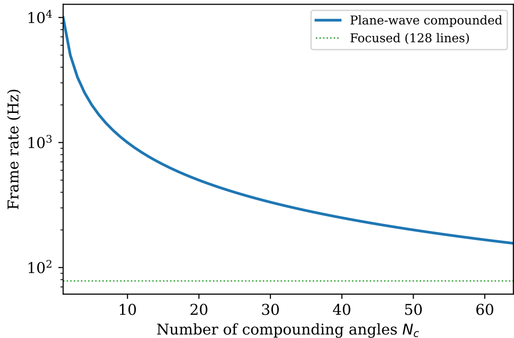
Frame Rate vs Compounding Angles (PRF = 10 kHz)
