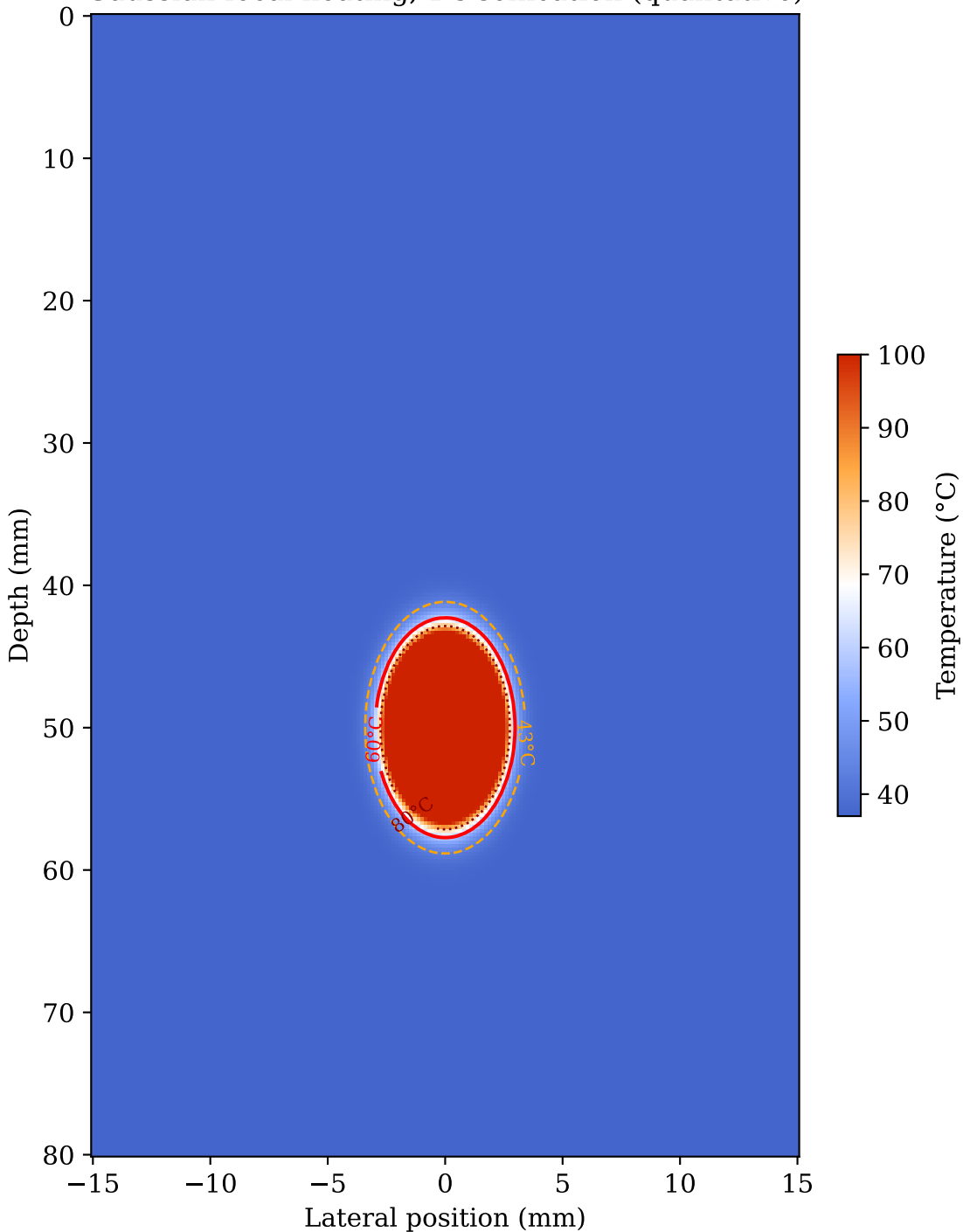
Thermal Ablation Zone — HIFU, f_0 = 1 MHz Gaussian focal heating, 1 s sonication (qualitative)
