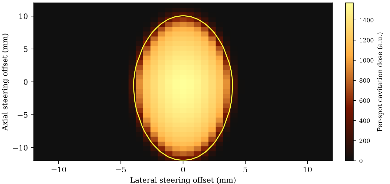
(D) Per-subspot dose vs electronic steering + attenuation yellow = treatable envelope ( \geq goal); 22% of raster reaches goal
