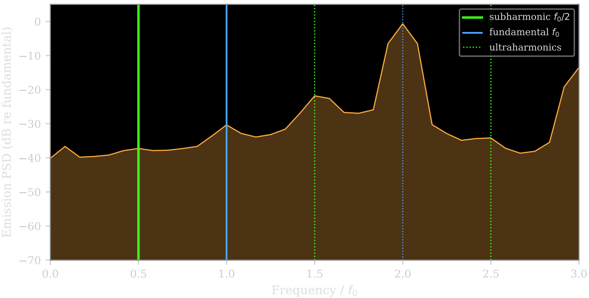
(A) Acoustic spectrum — cavitation signatures sub/ultraharmonics = stable-cavitation markers; floor = broadband (inertial)
