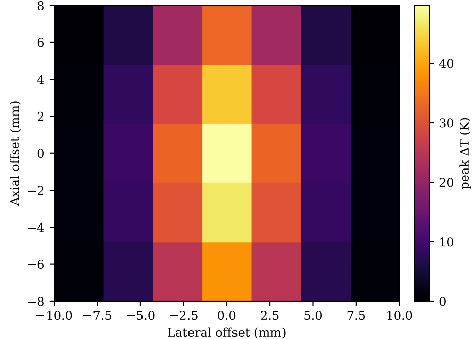
(B) Peak \Delta T /subspot — SEQUENTIAL max 49.7 K
