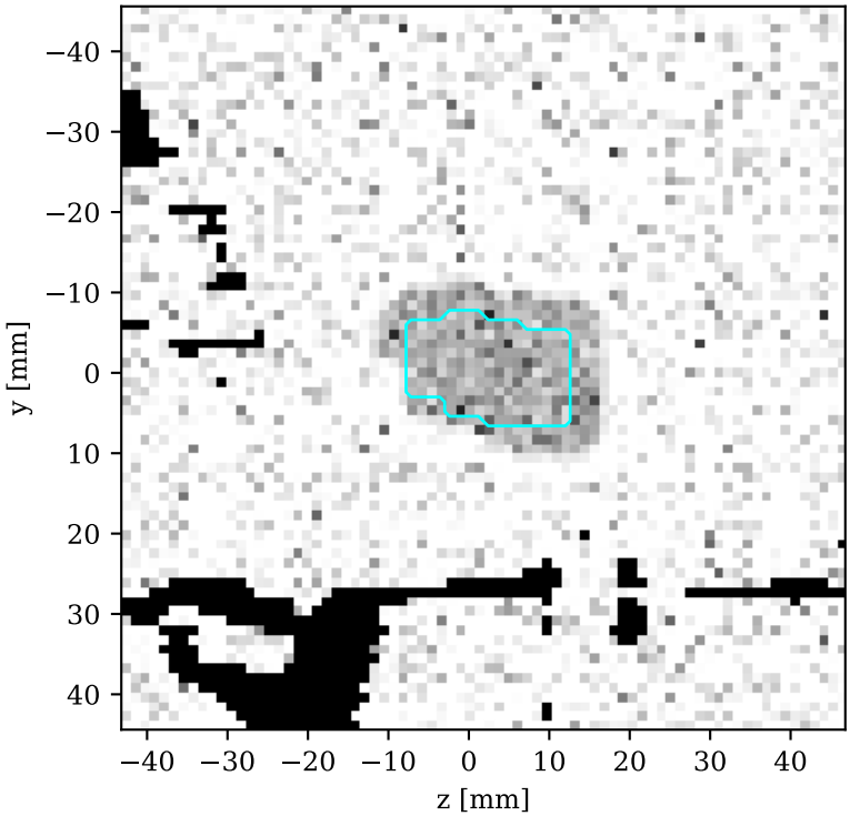
Biologically-effective dose (kill probability + LD iso-contours)
