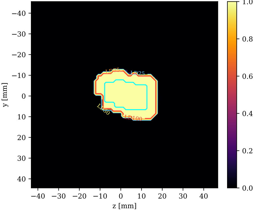
Biologically-effective dose (kill probability + LD iso-contours)
