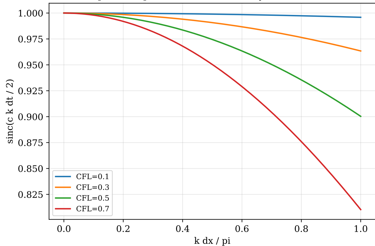
k-space temporal correction used by PSTD schemes
