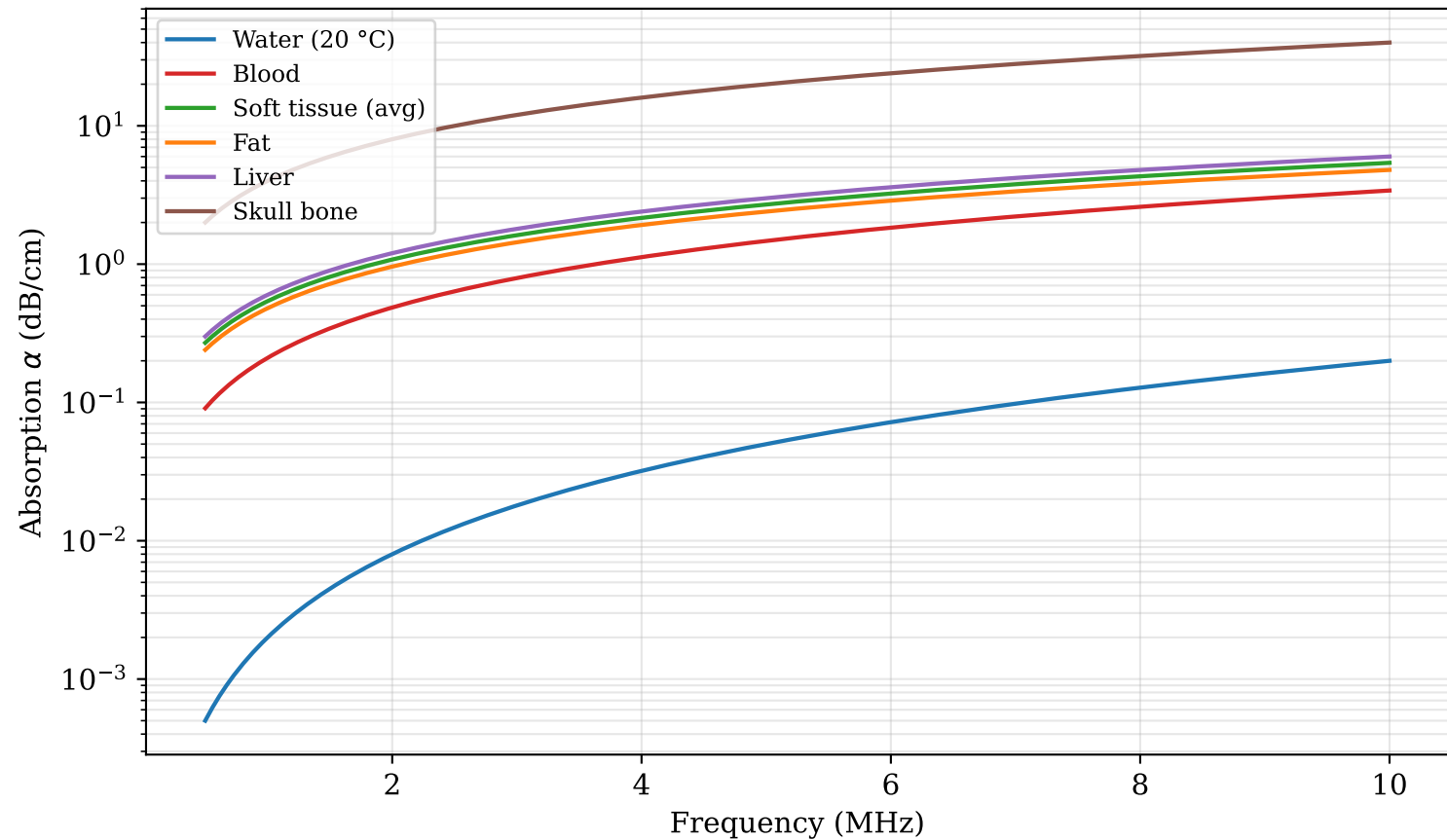
Power-law absorption: \alpha(f) = \alpha_0 f^y
