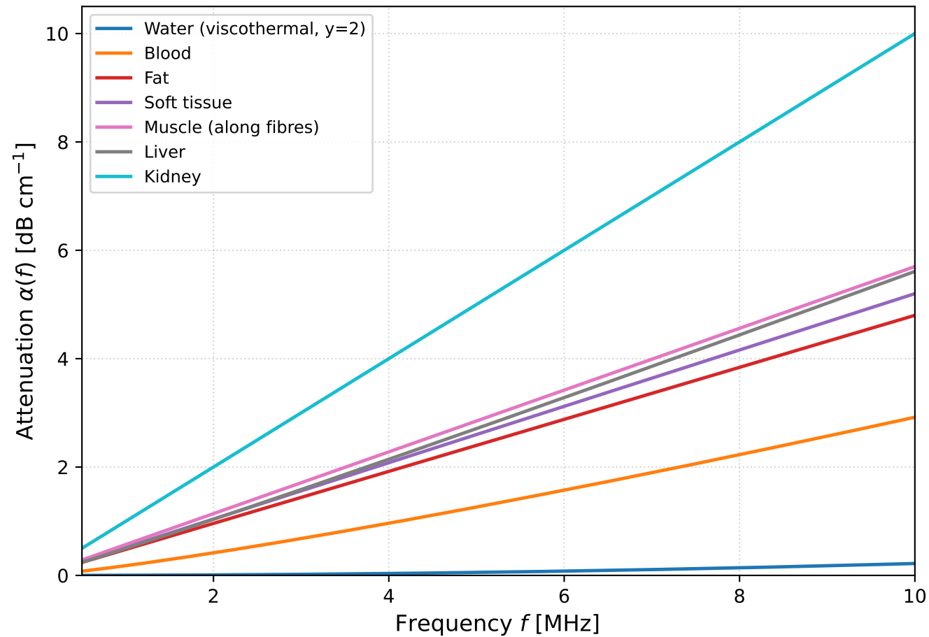
Figure 1.3 — Power-law attenuation \alpha(f) = \alpha_0 f^y (Duck 1990)
