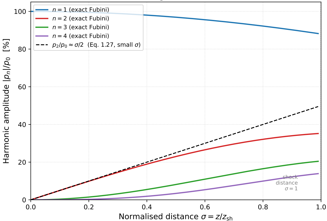
Figure 1.4 — Exact Fubini harmonic generation and the quasi-linear tangent (Theorem 1.8) lossless plane wave; p_2 grows as \frac{1}{2}\sigma near the source, then saturates as \sigma \rightarrow 1
