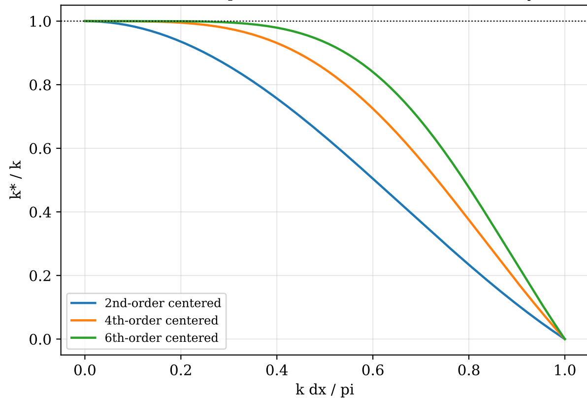
Finite-difference dispersion from modified-wavenumber symbols
