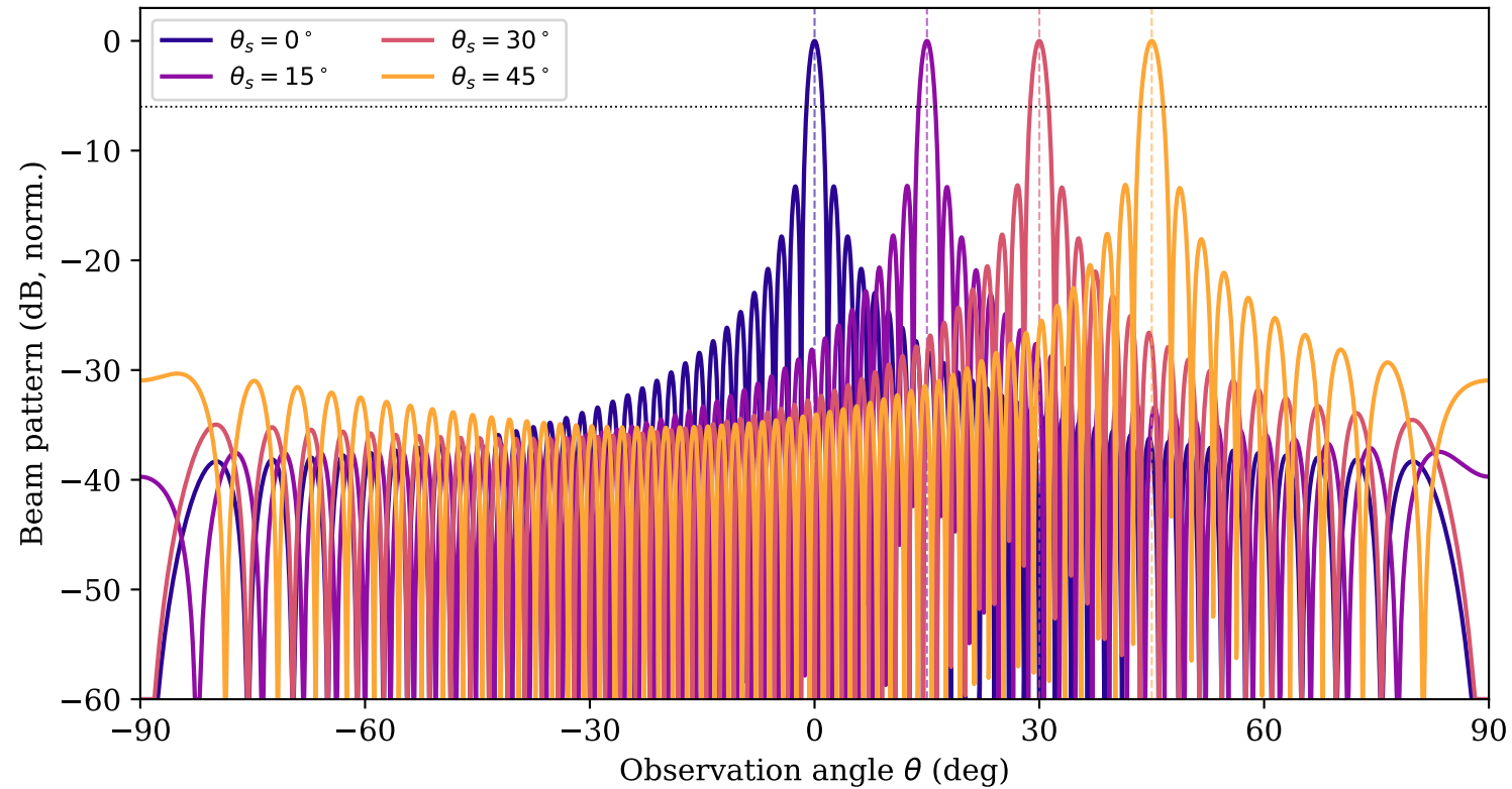
Electronic Steering with d = \lambda/2 : main lobe tracks \theta_s , no grating lobes
