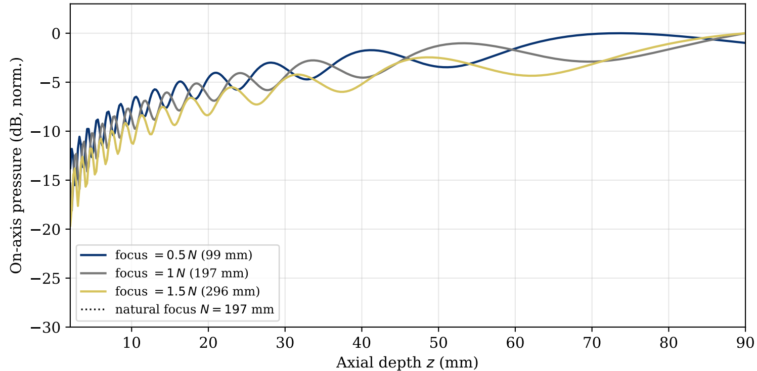
Focusing Around the Natural Focus N = D^2/(4\lambda) focal gain saturates as the focal range approaches N
