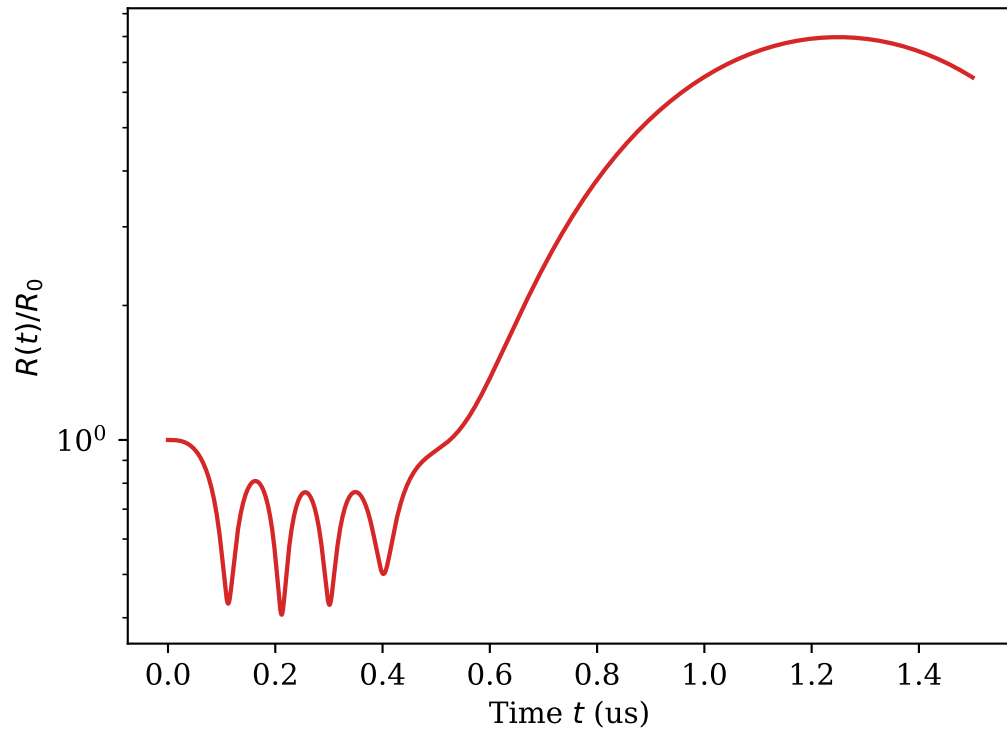
Inertial collapse detail ( P_{ac} = 1.5\text{ MPa} )
