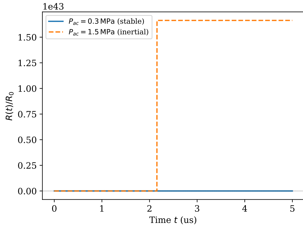
Rayleigh-Plesset dynamics, R_0 = 2\text{ }\mu\text{m} , f = 1\text{ MHz}
