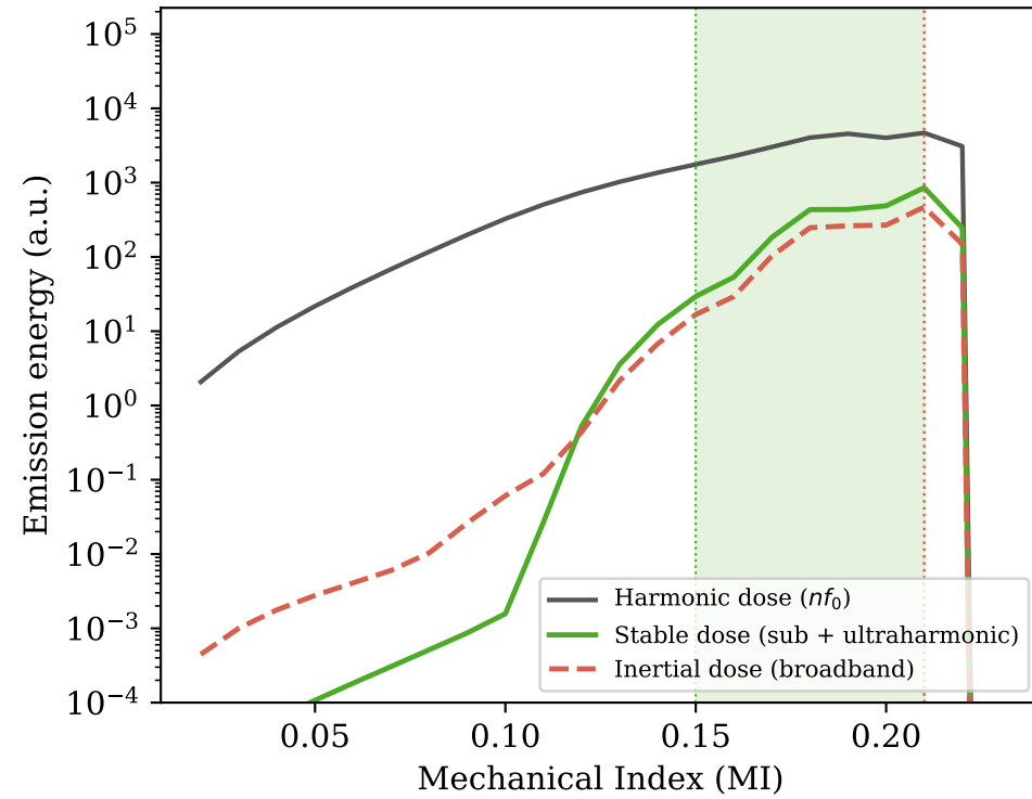
(B) Cavitation dose vs MI green band = stable-cavitation BBB window (MI 0.15–0.21) (C) Closed-loop dose controller pressure parks below inertial onset; stable dose accrues
