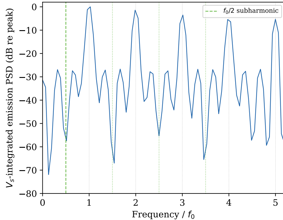
(A) PCD emission spectrum over V_s |p| = 170 kPa (MI = 0.17)
