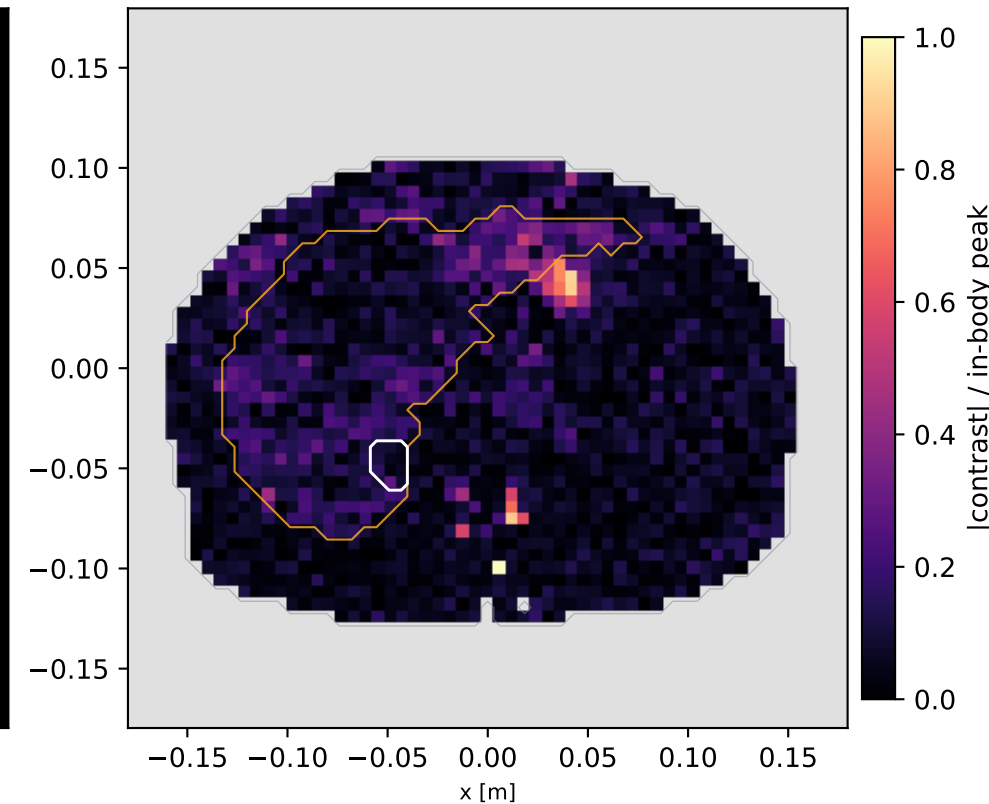
Reconstructed image (linearised Born, single-pass H^1 -Tikhonov) in-body peak = 0.183 (a.u.), multi-frequency imaging transmit, same aperture
