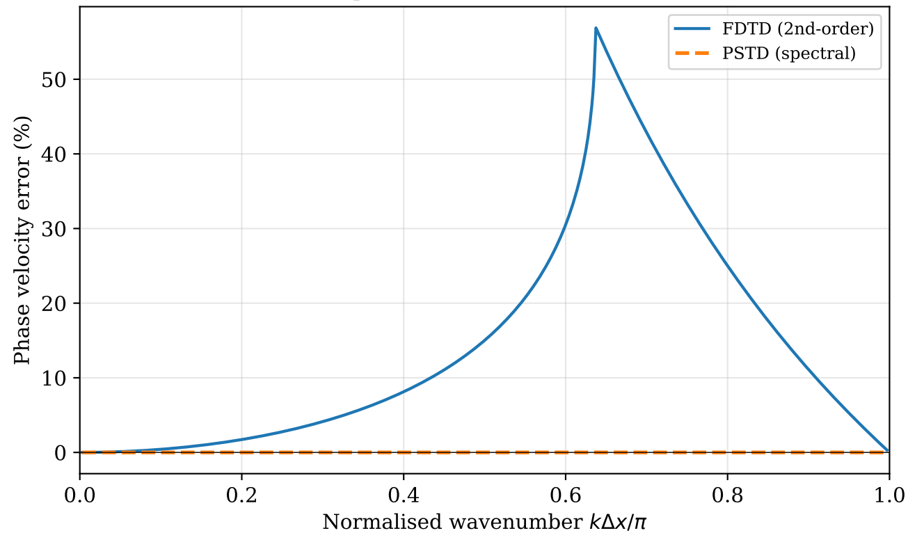
Numerical dispersion: PSTD vs second-order FDTD
